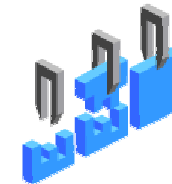
Messaging/JMS
