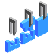
Messaging/JMS
