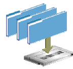
Content Repositories
