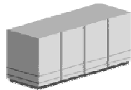
Legacy/ Mainframe
