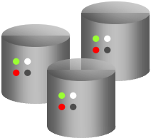
Databases
