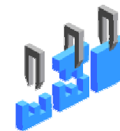
Messaging/JMS
