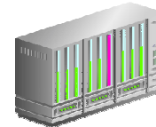
Mainframes
