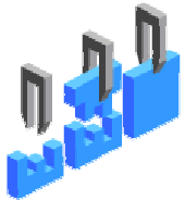
Middleware
