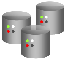
Databases
