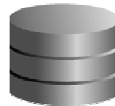
Databases
